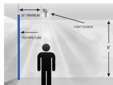
Recommended setback distance between artificial light source (non-LED) and PEX pipe/tubing in a typical residential or light commercial setting
