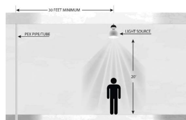
Recommended setback distance between artificial light source (non-LED) and PEX in a typical industrial setting
